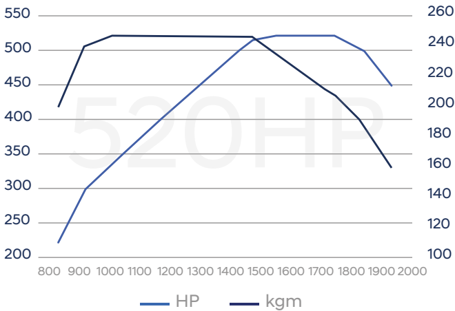
XCIENT GT EURO 5 (SCR) D6C F52
